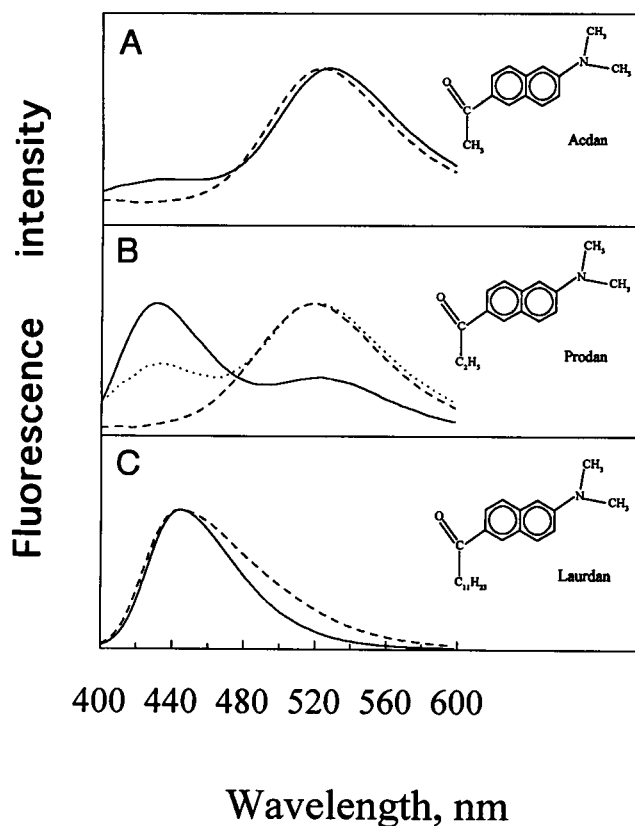
FIGURE 4 Effect of ethanol on the emission spectra of Acдан (A), Prodan (B), and Laurdan (C) fluorescence at 20°C. [DPPC] is 1.17 mM for all the samples except for the dotted line, which was obtained from a sample with [DPPC] = 0.48 mM. The solid and dotted lines represent samples without ethanol, and the dashed line represents samples containing 1.8 M ethanol.
