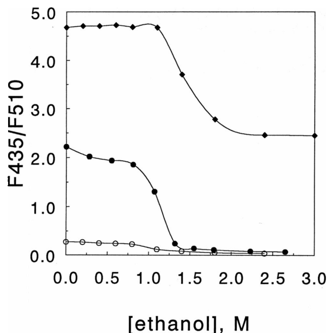
FIGURE 5 Effect of ethanol on F_{435}/F_{510} of Acдан (○), Prodan (●), and Laurdan (◆) fluorescence in DPPC multilamellar vesicles. F_{435}/F_{510} is the ratio of the fluorescence intensity at 435 nm to that at 510 nm. [DPPC] = 1.17 mM and the probe-to-lipid ratio is <1/500. Temperature = 20°C.
